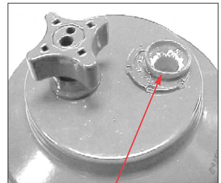
Sensor Port with Plastic Drain Plug (Must be replaced prior to service)
